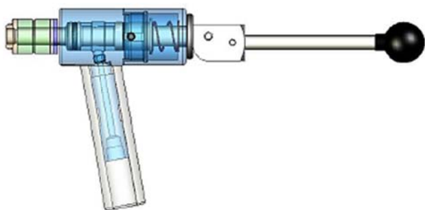
HIH Type - Fill Port with Handle
